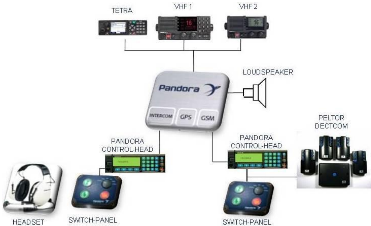
Overview of the Swedish Sea Rescue Societys standard Telium Pandora-system.
